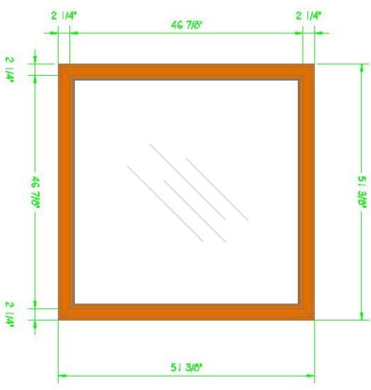
PLAN (INTERIOR SIDE)
